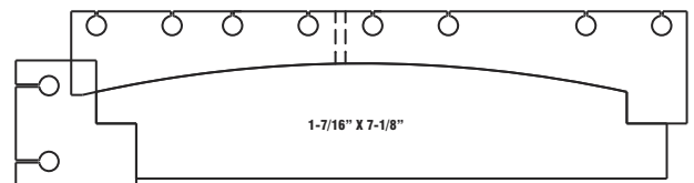
Log Cabin Siding 9
