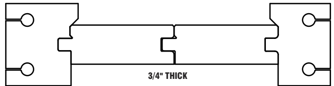
Tongue & Groove Flooring 6
