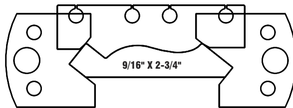
Crown 6-8 (same profile different widths)
