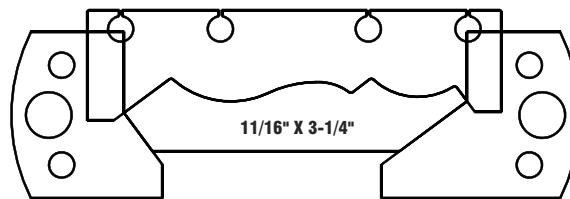
Crown 1-5 & 10 (same profile different widths)
